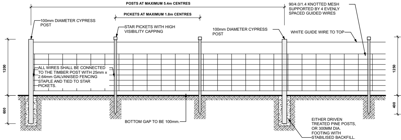
ELEVATION: POST AND WIRE FENCE
