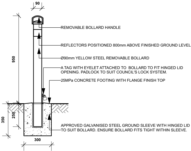
SECTION : REMOVABLE STEEL BOLLARD
