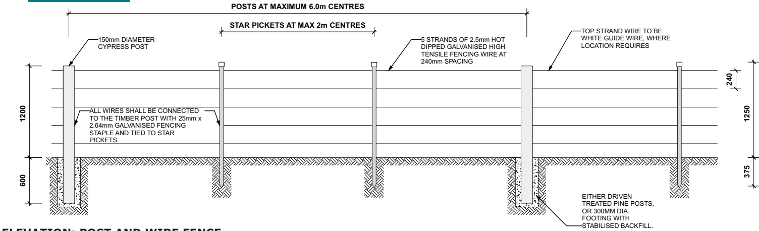
ELEVATION: POST AND WIRE FENCE
