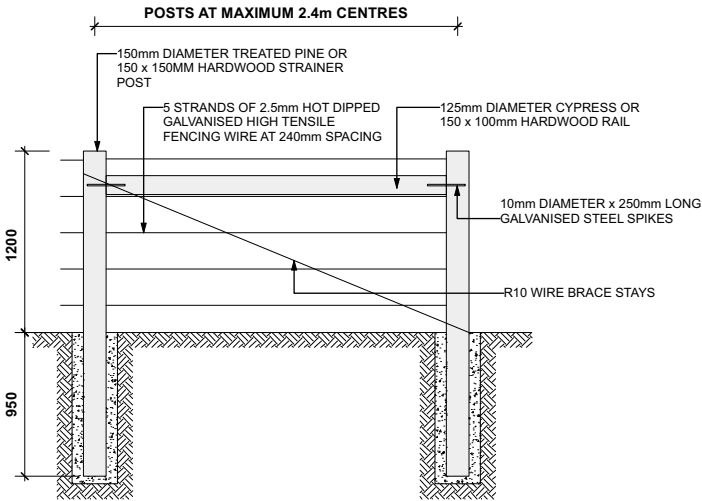
ELEVATION: STRAINER POST ASSEMBLY AND CORNER
